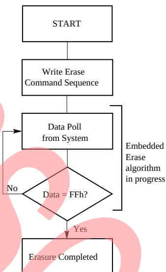
Figure 12.2 Erase Operation
