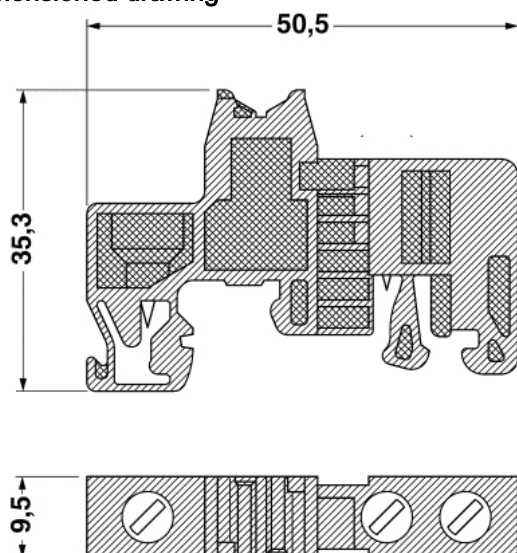
Dimensioned drawing
