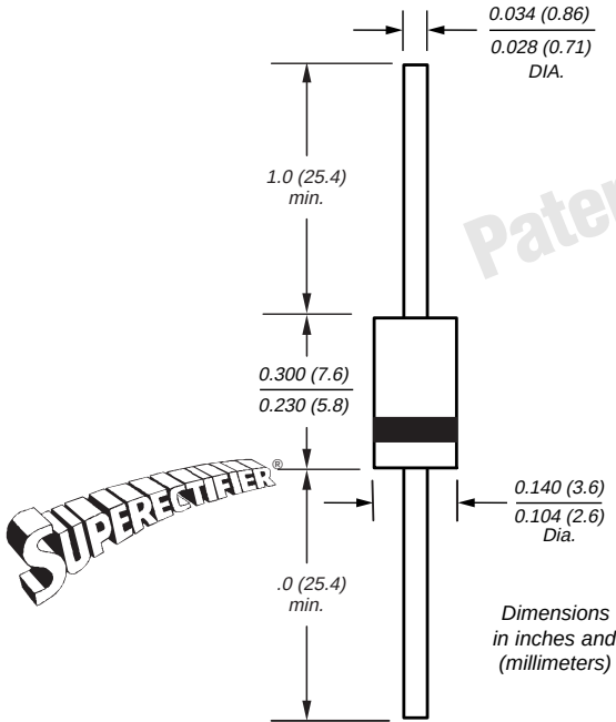
DO-204AC (DO-15)
