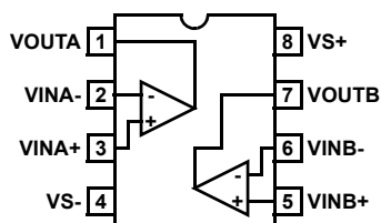
EL1516 (8 LD SOIC, 8 LD MSOP) TOP VIEW
