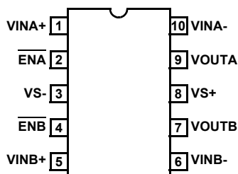
EL1516A (10 LD MSOP) TOP VIEW
