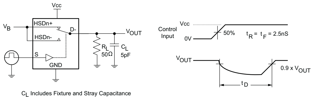
Figure 2. Break-Before-Make Timing
