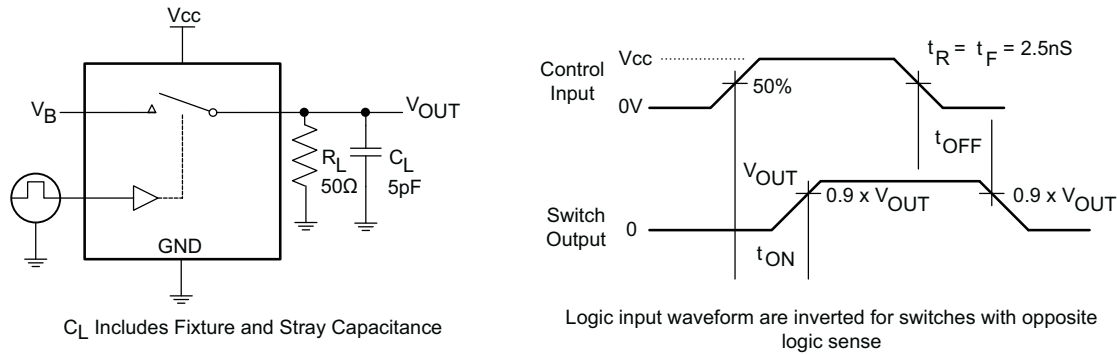
Figure 1. Turn-On/Turn-Off Timing
