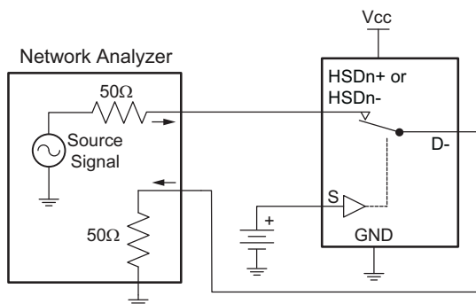
Figure 5. Bandwidth
