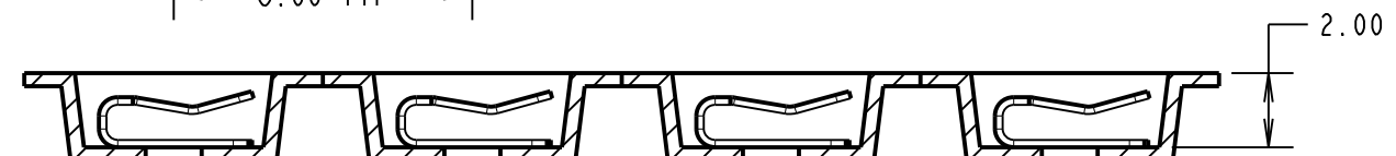
SECTION Y-Y
