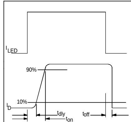
Figure 8. Delay Time Definitions
