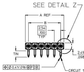
DETAIL Z SCALE 5:1
