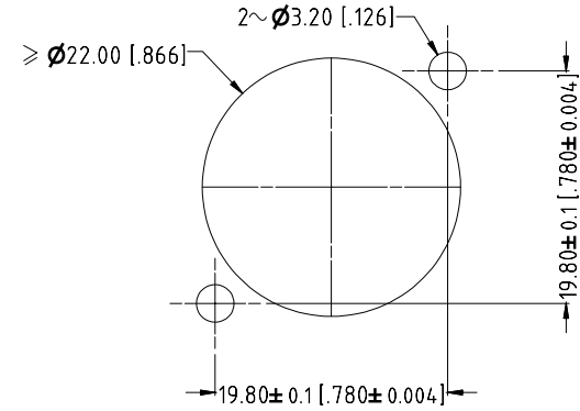
PANEL CUT OUT REAR VIEW
