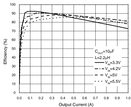
Figure 5. Efficiency vs. Output Current ( V_{OUT}=2.5V )
