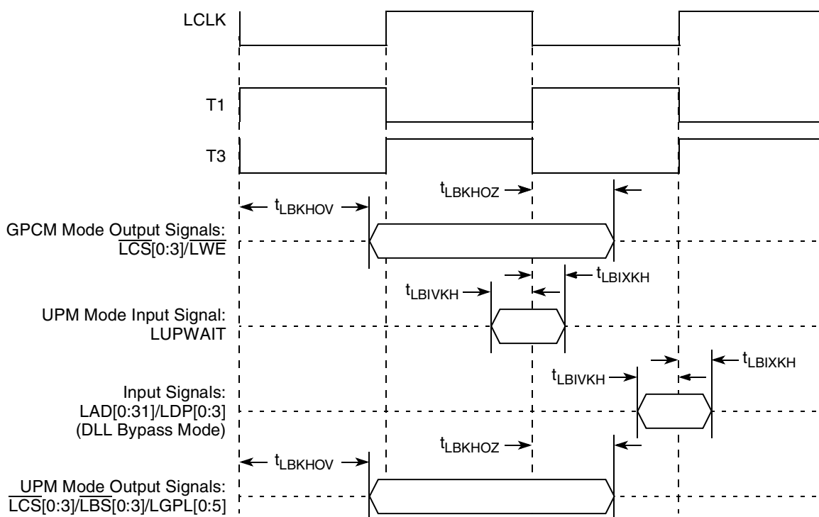
Figure 25. Local Bus Signals, GPCM/UPM Signals for \text{LCRR}[\text{CLKDIV}] = 2 (DLL Bypass Mode)
