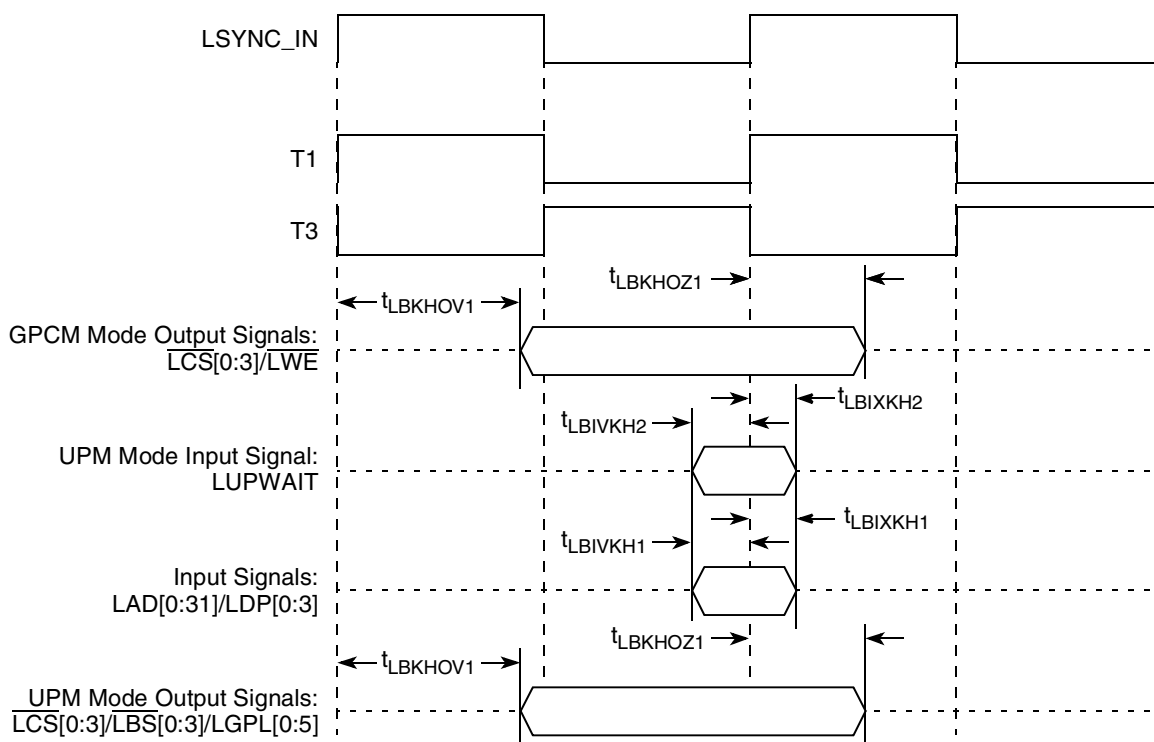
Figure 24. Local Bus Signals, GPCM/UPM Signals for \text{LCRR}[\text{CLKDIV}] = 2 (DLL Enabled)
