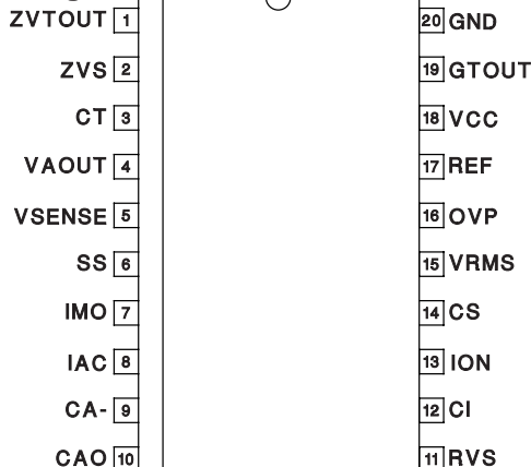
SOIC-20 (Top View) DW Package
