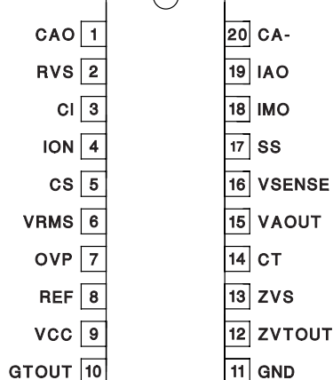
DIL-20 (Top View) J or N Package
