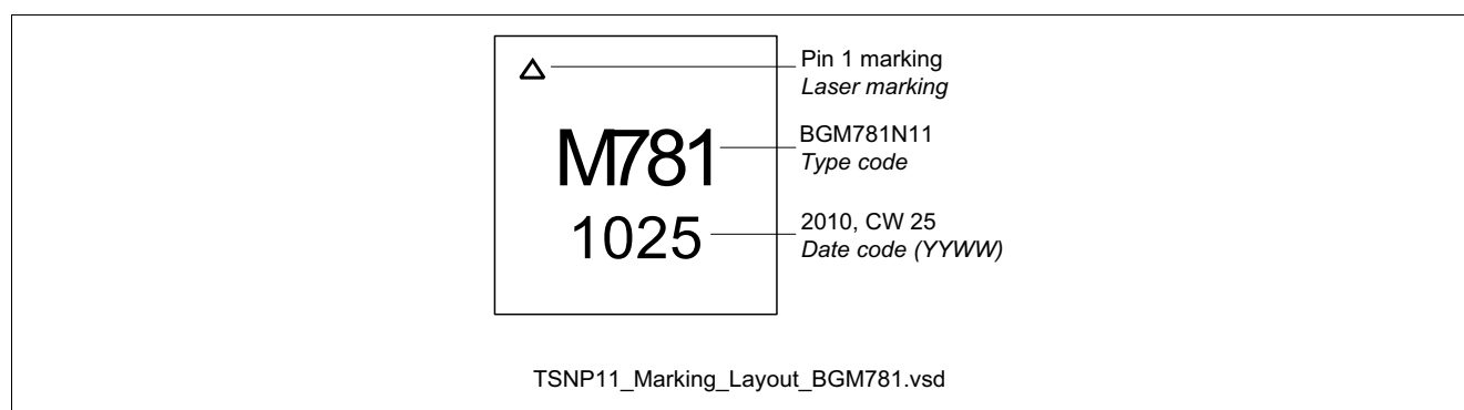
Figure 6 Marking layout
