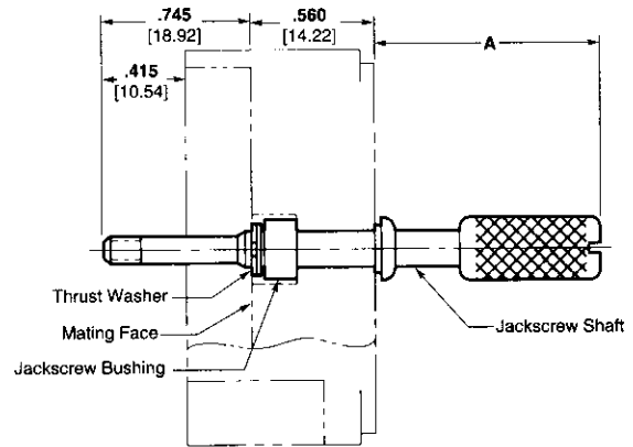
Male Turnable Jackscrew
