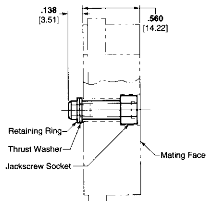
Fixed Female Jackscrew
