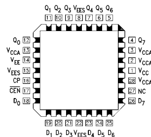
28-Pin PLCC
