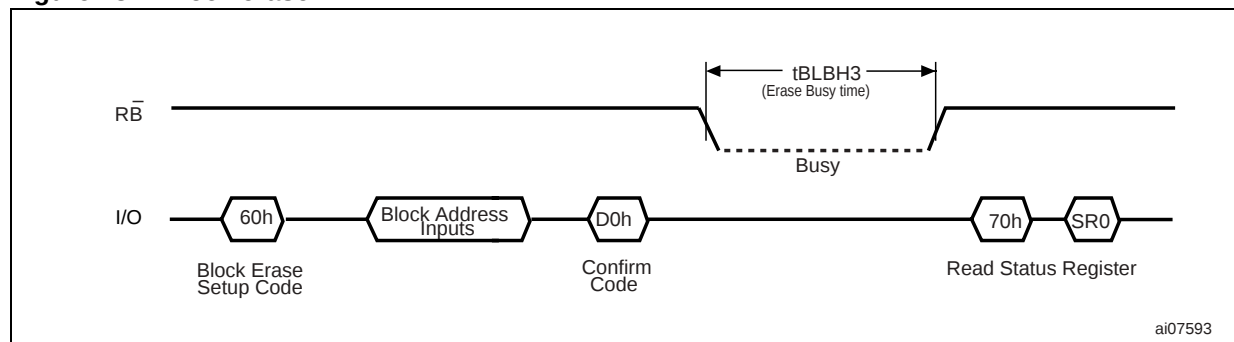
Figure 18. Block erase
