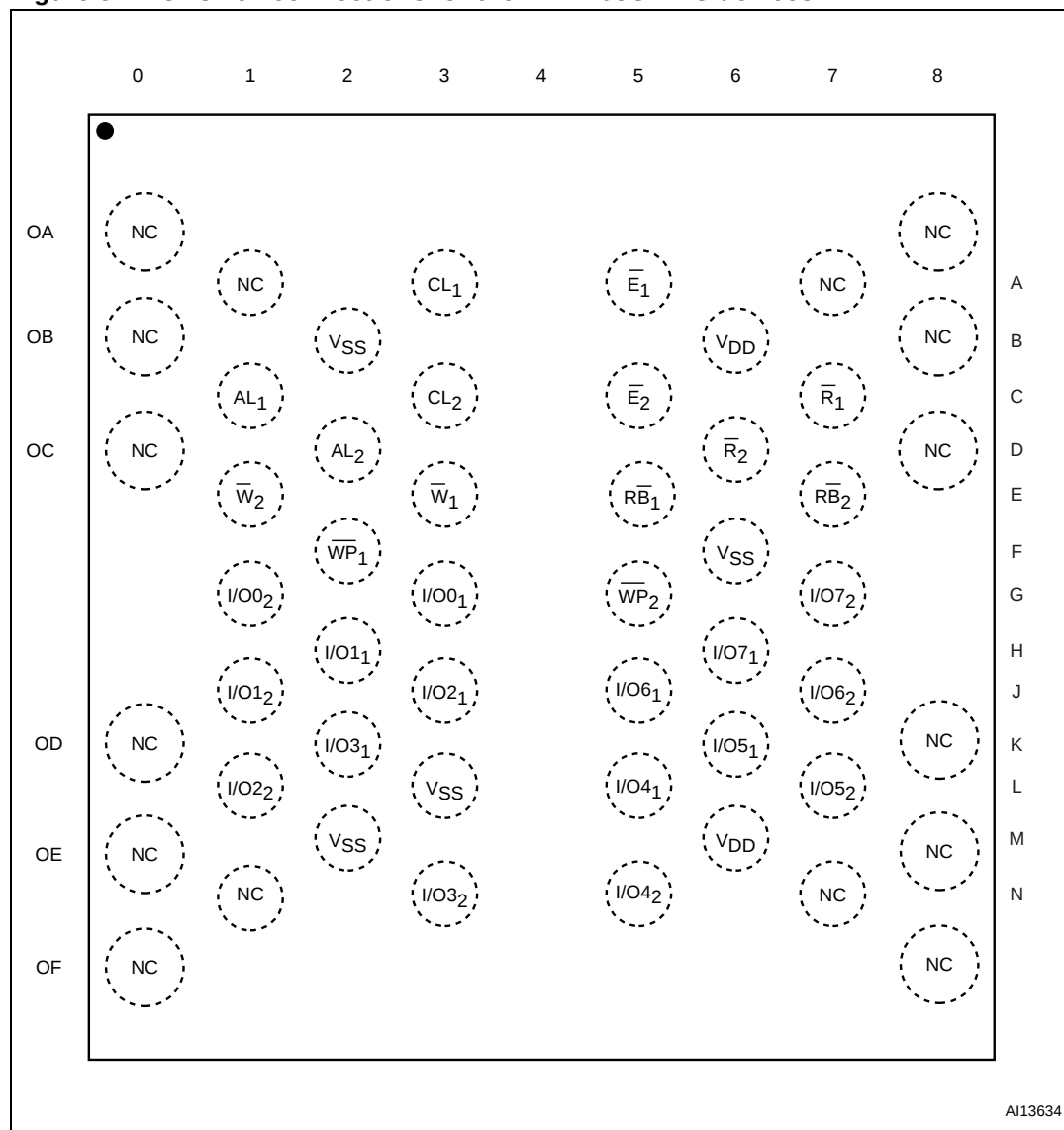
Figure 5. ULGA52 connections for the NAND08G-B4C devices
