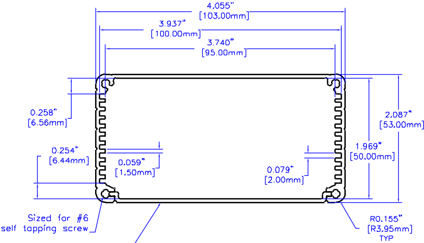
EXTRUSION
