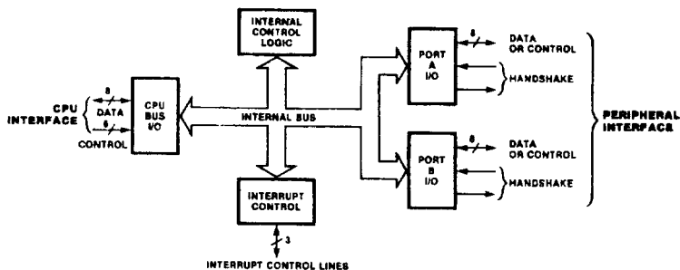
Figure 3 : Block Diagram.
