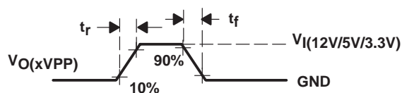
Rise/Fall Time (xVPP)
