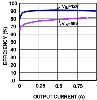
Efficiency @ V_{OUT}=5V L1=15\mu H , f_s=500kHz
