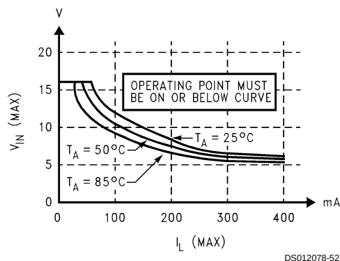
FIGURE 6. Safe Operation Boundary Curves for Figure 5
