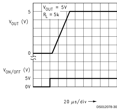
Turn-On Waveform
