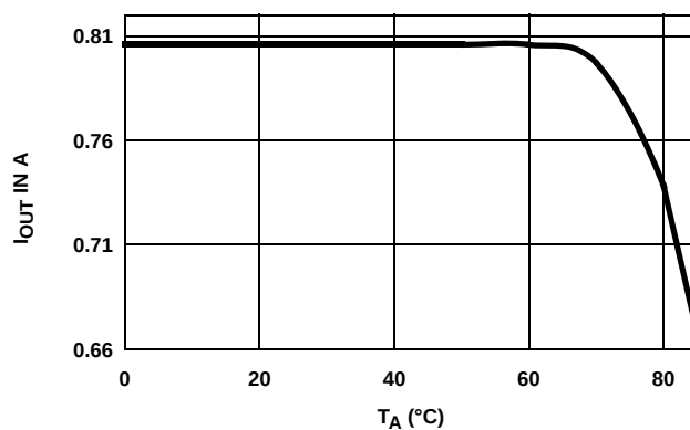
FIGURE 3. OUTPUT CURRENT DERATING 40 LD 6x6 QFN: I_{OUT\_max} vs T_A
