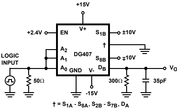
FIGURE 3B. DG407 TEST CIRCUIT
