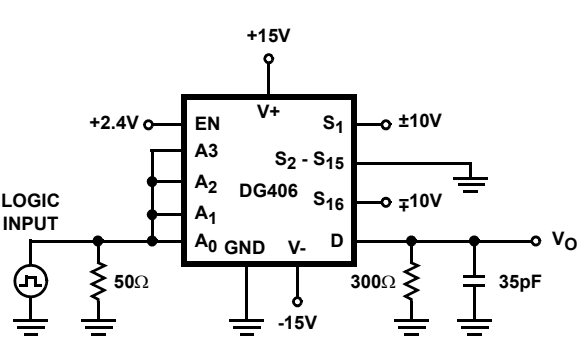
FIGURE 3A. DG406 TEST CIRCUIT
