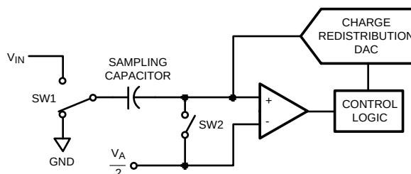
Figure 19. ADC081S101 in Hold Mode
