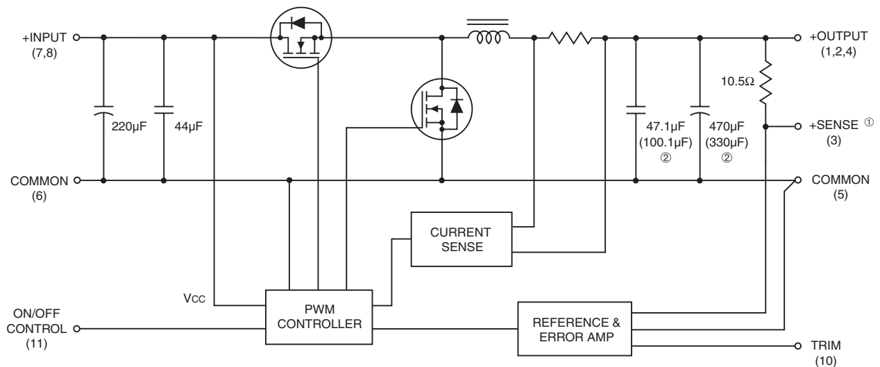
Figure 1. Simplified Schematic
