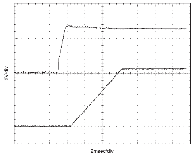
Power-Up From V_{IN} ( V_{IN} = 5V , V_{OUT} = 3.3V/10A , C_{IN} = 220\mu F , No External C_{OUT} )
