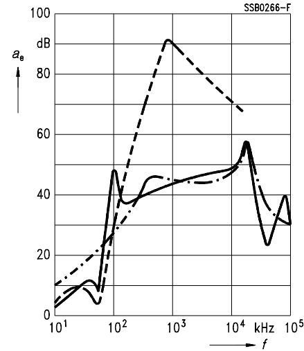
B84114-D-*60
