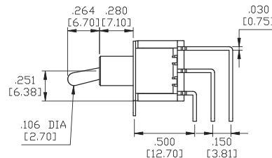
M7 Double Pole .244 DIA [6.20]
