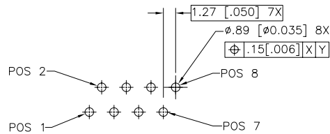
VIEW C SCALE 2/1 TYPICAL FOOTPRINT
