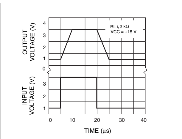
Figure 4. Voltage follower pulse response with V_{CC} = 15\text{ V}
