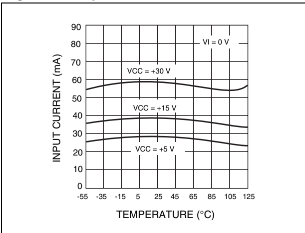
Figure 6. Input current
