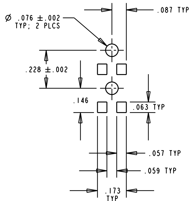
SOLDER PAD/HOLES LAYOUT SINGLE COLOR LED 597-3XX1-5XX
