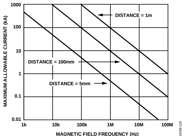
Figure 26. Maximum Allowable Current for Various Current-to- ADuM5200W/ADuM5201W/ADuM5202W Spacings
