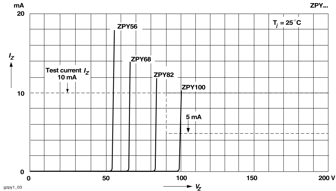
Figure 9. Breakdown Characteristics
