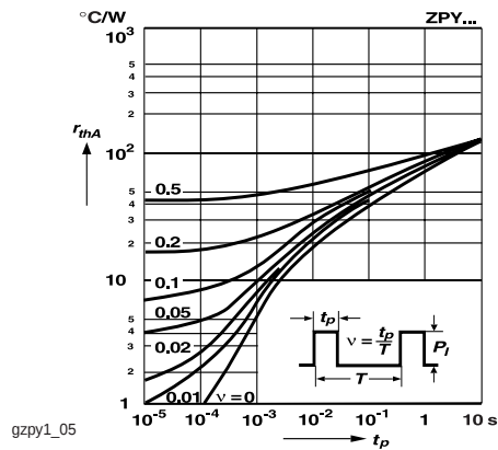
Figure 2. Pulse Thermal Resistance vs. Pulse Duration
