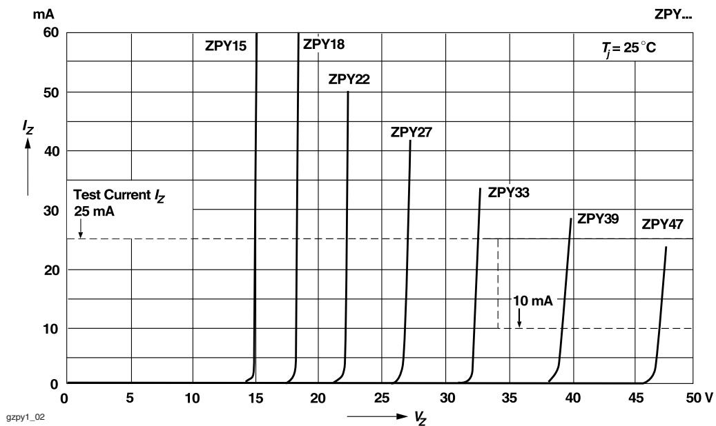
Figure 8. Breakdown Characteristics
