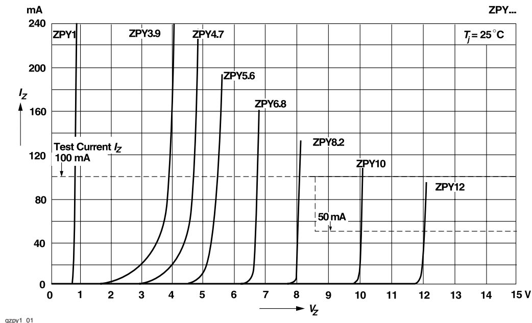
Figure 7. Breakdown Characteristics
