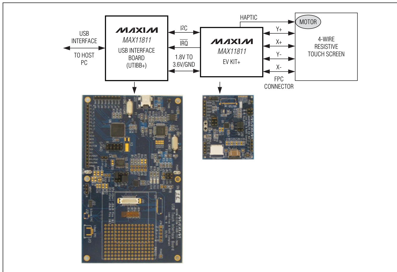
Figure 2. MAX11811 Touch Evaluation System (TEVS) Block Diagram
