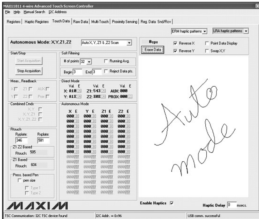
Figure 9. Touch Data Tab (Autonomous Mode)
