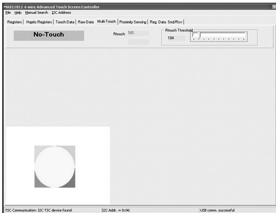
Figure 11. Multi-Touch Tab (Before Zoom Out and Rotate)
