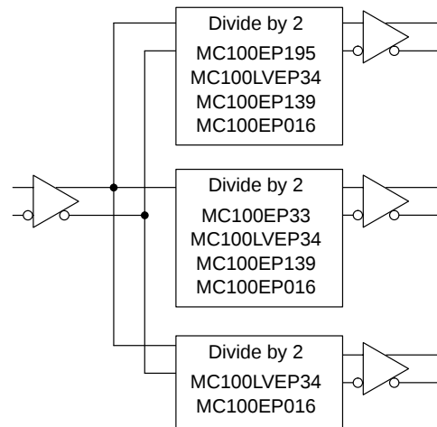
Figure 8. Example of Clock Division
