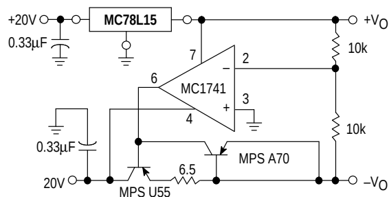
Figure 7. \pm 15 \text{ V} Tracking Voltage Regulator
