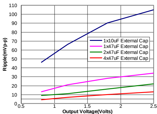
Figure 48. Output ripple voltage for various output voltages with external 1x10 \mu F, 1x47 \mu F, 2x47 \mu F or 4x47 \mu F ceramic capacitors at the output (30A load). Input voltage is 12V.
