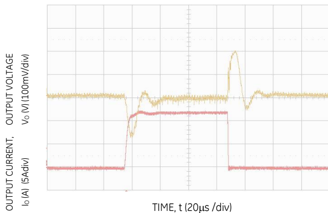
Figure 3. Transient Response to Dynamic Load Change from 0% to 50% to 0% of full load with V_{IN} = 12V .
