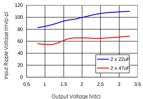
Figure 47. Input ripple voltage in mV, p-p for various output voltages with 2x22 \mu F or 2x47 \mu F ceramic capacitors at the input (30A load). Input voltage is 5V.
