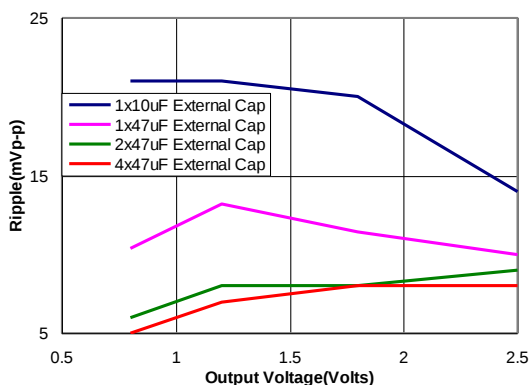
Figure 49. Output ripple voltage for various output voltages with external 1x10 \mu F, 1x47 \mu F, 2x47 \mu F or 4x47 \mu F ceramic capacitors at the output (30A load). Input voltage is 5V.
