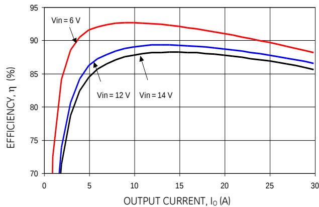
Figure 10. Converter Efficiency versus Output Current.
