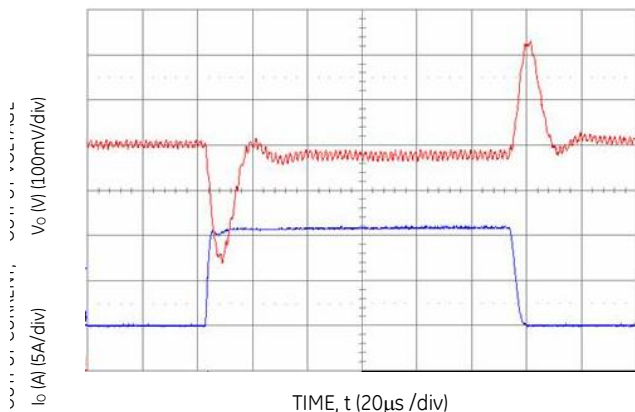
Figure 21. Transient Response to Dynamic Load Change from 0% to 50% of full load with V_{IN}=12V .
