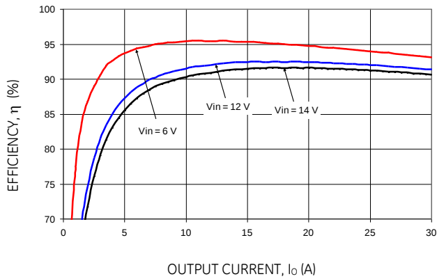
Figure 16. Converter Efficiency versus Output Current.
