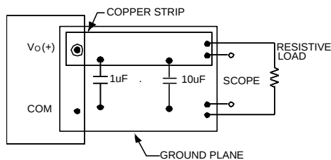
Figure 43. Input Reflected Ripple Current Test Setup.
