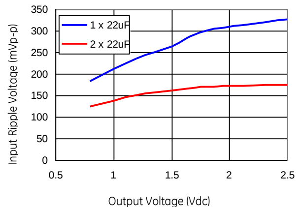
Figure 46. Input ripple voltage for various output voltages with 1x22 \mu F or 2x22 \mu F ceramic capacitors at the input (30A load). Input voltage is 12V.
