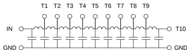
Functional Diagram
