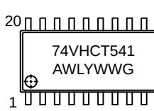
SOEIAJ-20 SUFFIX M CASE 967
