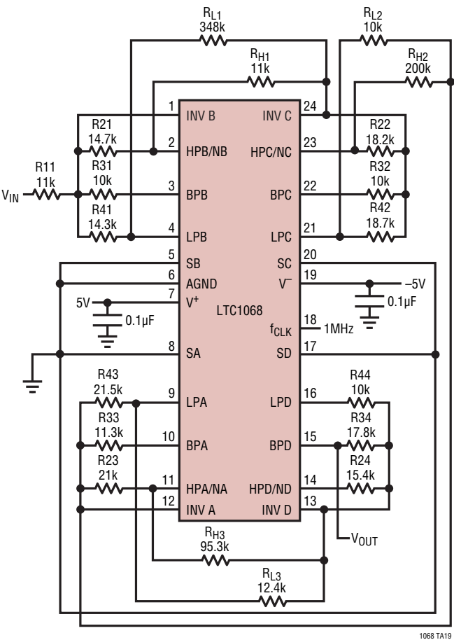
24-Lead Package
