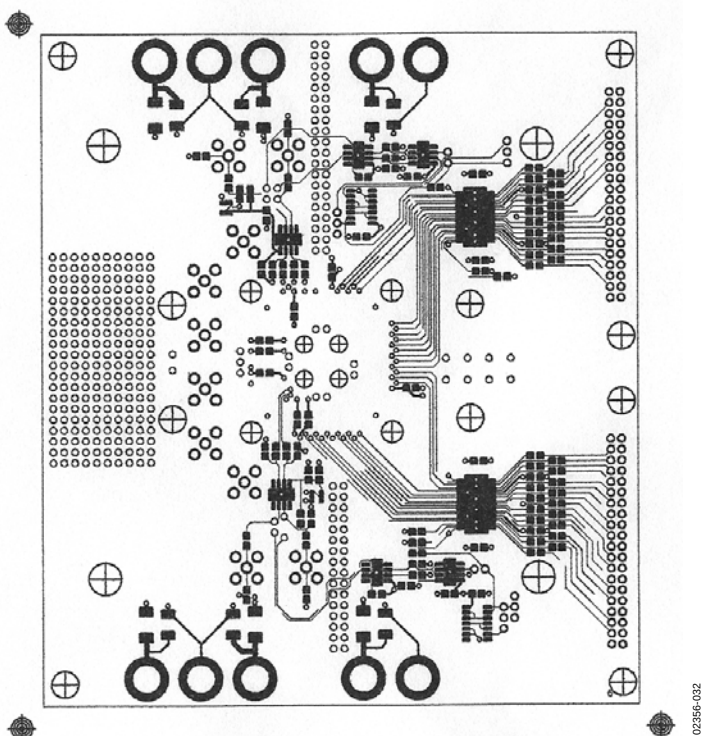
Figure 32. Bottom Layer Copper
