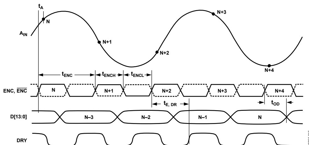
Figure 2. Timing Diagram
