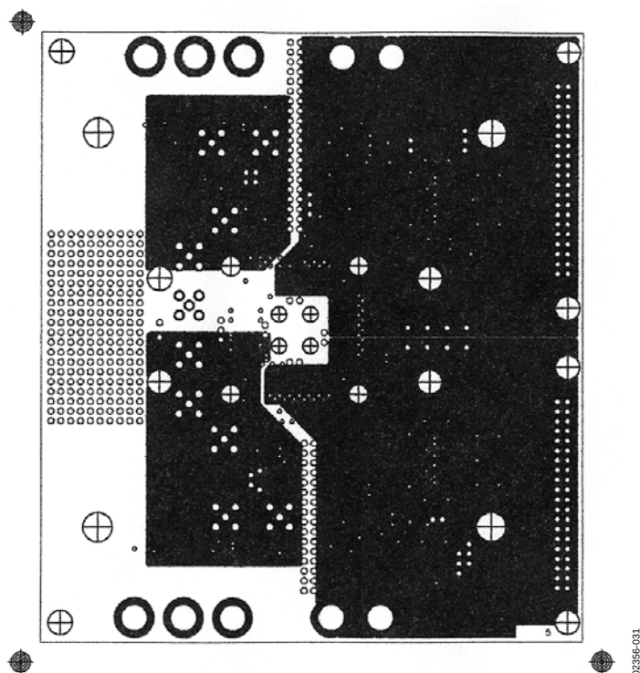
Figure 31. Fifth Layer Copper
