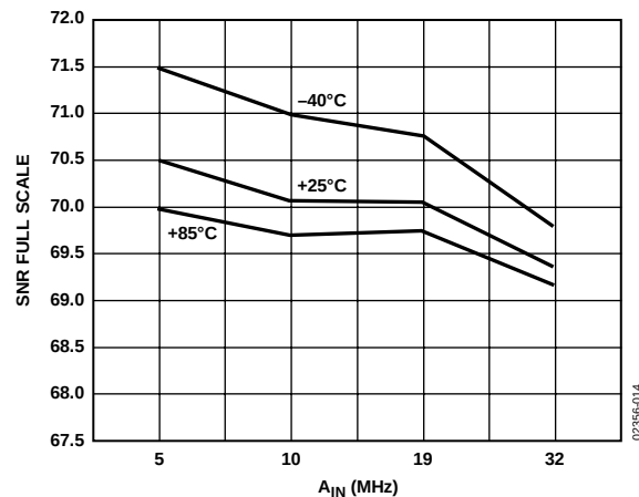
Figure 19. SNR vs. A_{IN} Frequency
