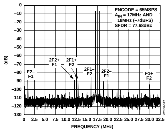
Figure 17. Two Tone @ 17 MHz and 18 MHz
