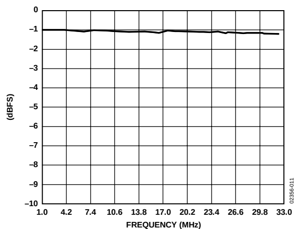
Figure 16. Gain Flatness
