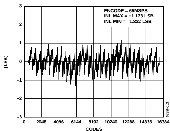
Figure 18. Integral Nonlinearity
