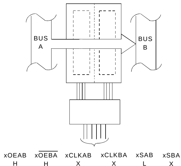
REAL-TIME TRANSFER BUS A TO B
