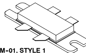
CASE 465M-01, STYLE 1 NI-780-4 MRF8HP21130HR3
