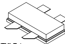
CASE 465H-02, STYLE 1 NI-780S-4 MRF8HP21130HSR3
