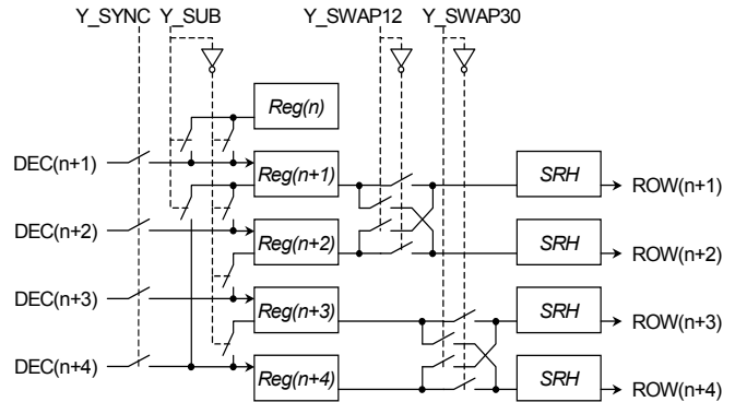
Figure 10. Row Structure
