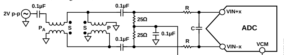
Figure 46. Differential Double Balun Input Configuration
