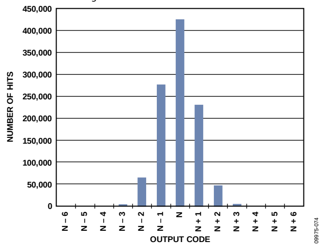
Figure 21. Shorted Input Histogram
