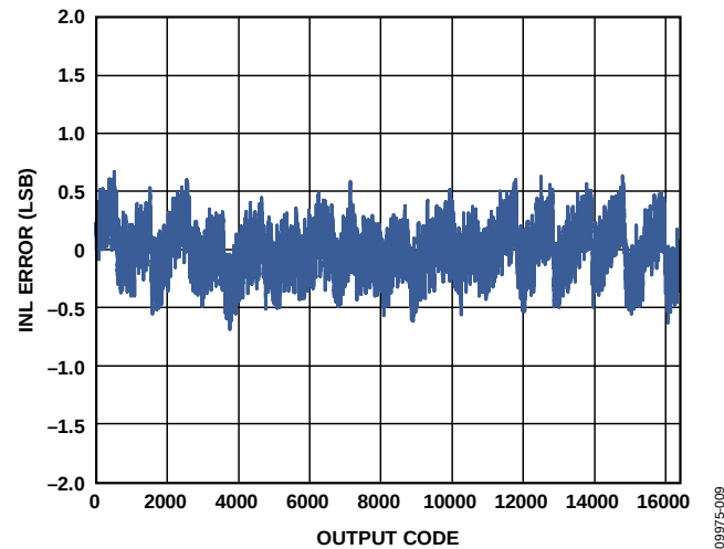
Figure 33. INL Error with f_{IN} = 9.7 MHz
