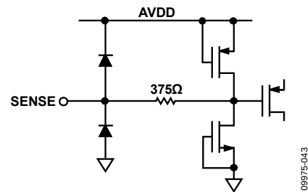
Figure 39. Equivalent SENSE Circuit
