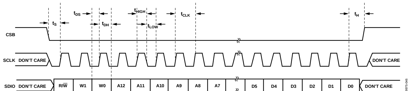
Figure 62. Serial Port Interface Timing Diagram
