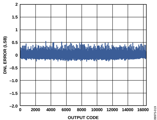
Figure 20. DNL Error with f_{IN} = 9.7 MHz
