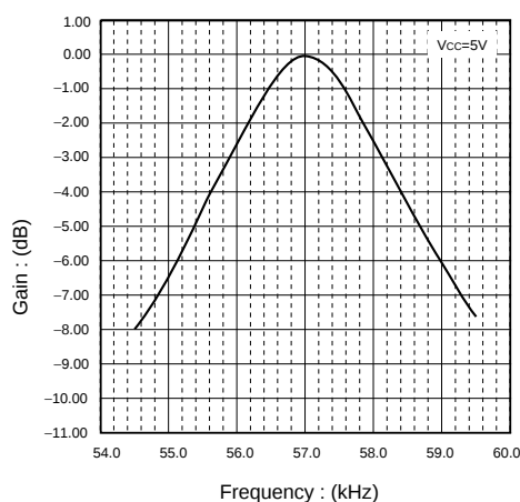
Fig.6 RPM7157 Series BPF Characteristics
