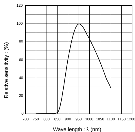
Fig.7 Relative spectral sensitivity of photo diode
