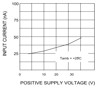
Figure 14: Input current
