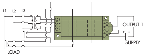
CR6230 CR6231 3 element - 3 Wire, 0 - 5 VDC Output shown with external voltage and current transformers
