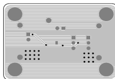
Figure 8. Bottom Layer
