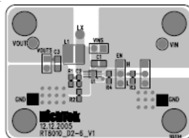
Figure 7. Top Layer
