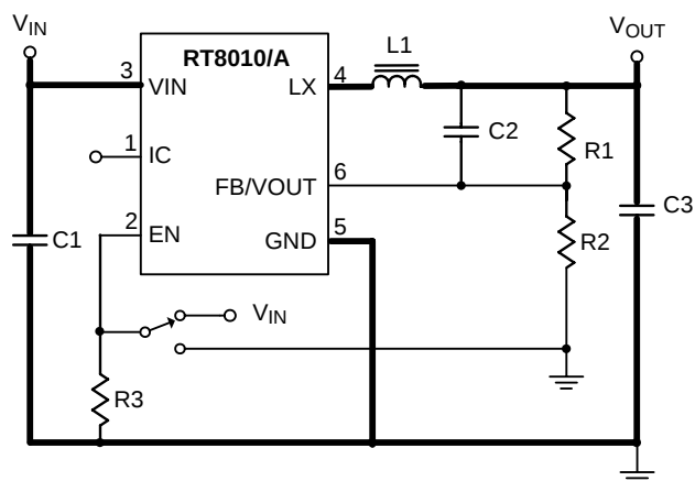
Figure 6. EVB Schematic
