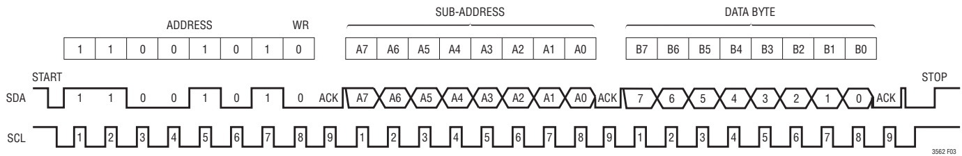
Figure 3. Bit Assignments
