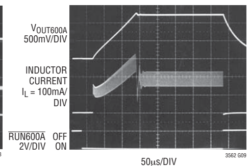
Start-Up Transient Pulse Skip Mode
