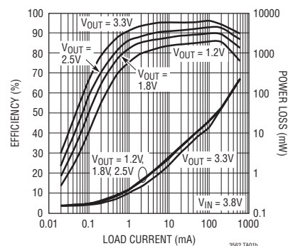
R600x Burst Mode Efficiency and Power Loss vs Load Current
