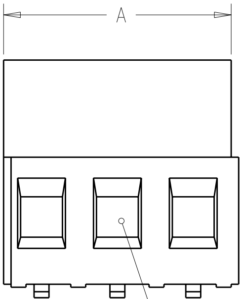
WIRE ENTRY
